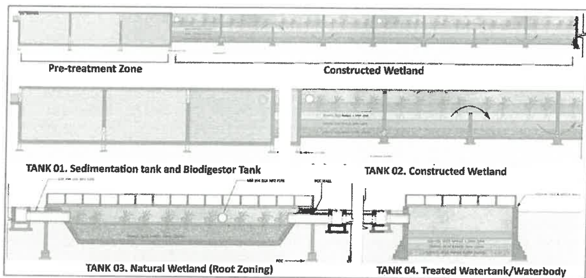
Figure 22: Process of Water Purification in a Constructed Wetland
