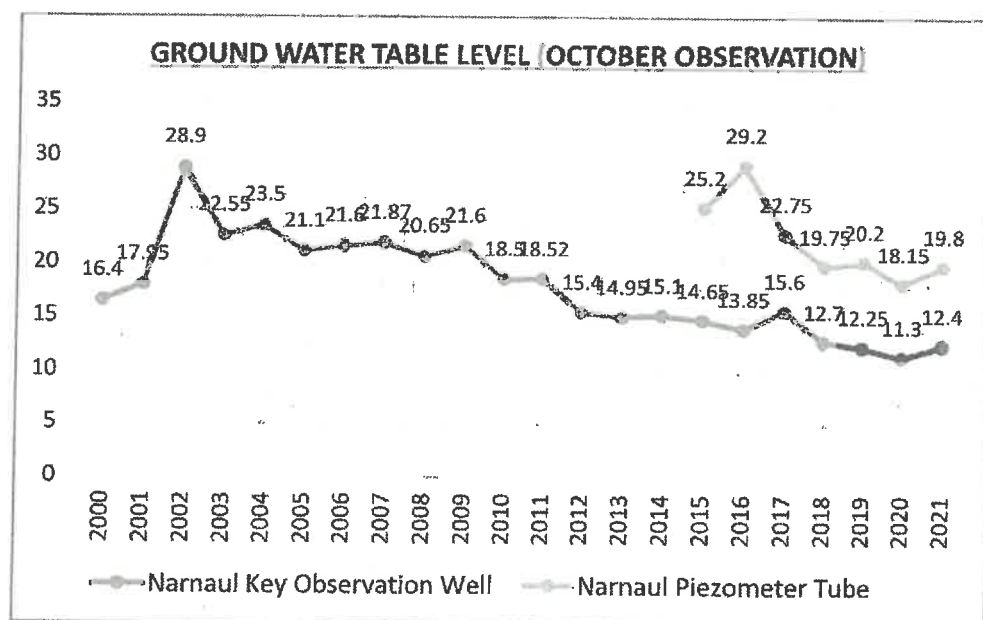
Figure 9: Groundwater Table Observation, October
