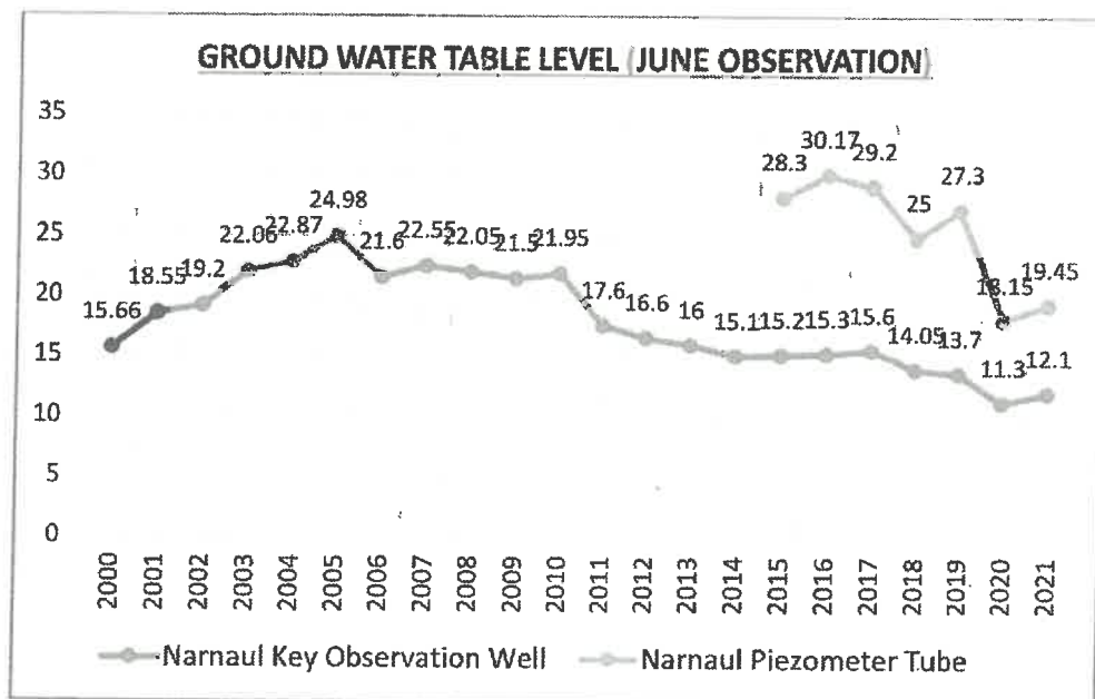
Figure 8: Groundwater Table Observation, June
