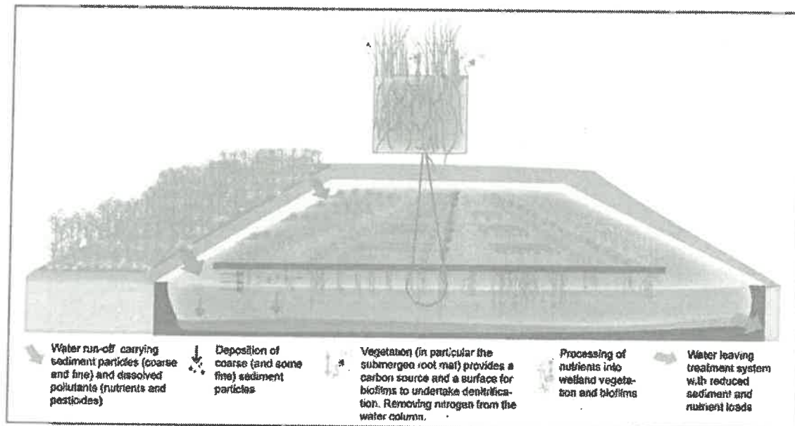
Figure 24: Working of Floating Wetlands
